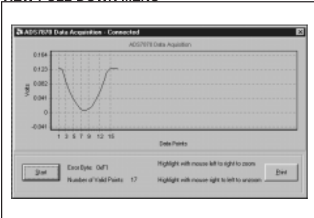
FIGURE 7. PGA Overload. Note that the number of valid data points will vary depending on the level of the sine wave at the time the data set is collected.
