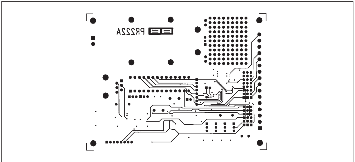
FIGURE 20. Bottom Side.
